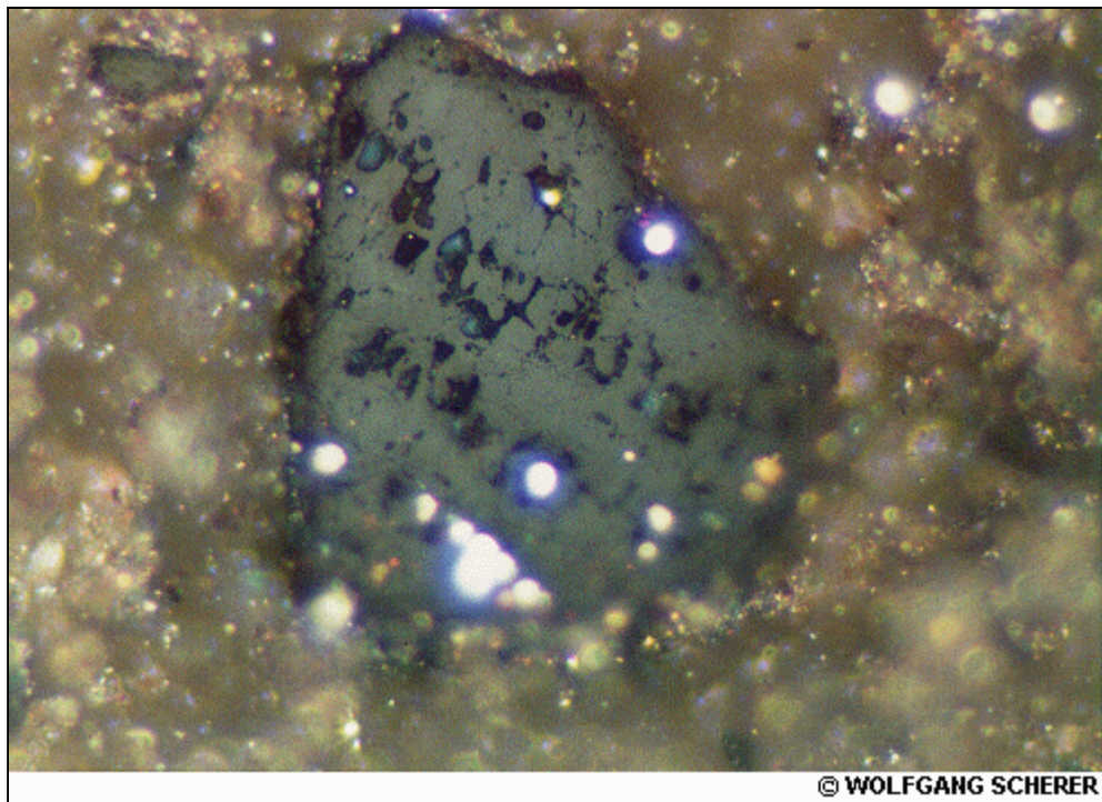
Sample ATP-30 Vitrinite
