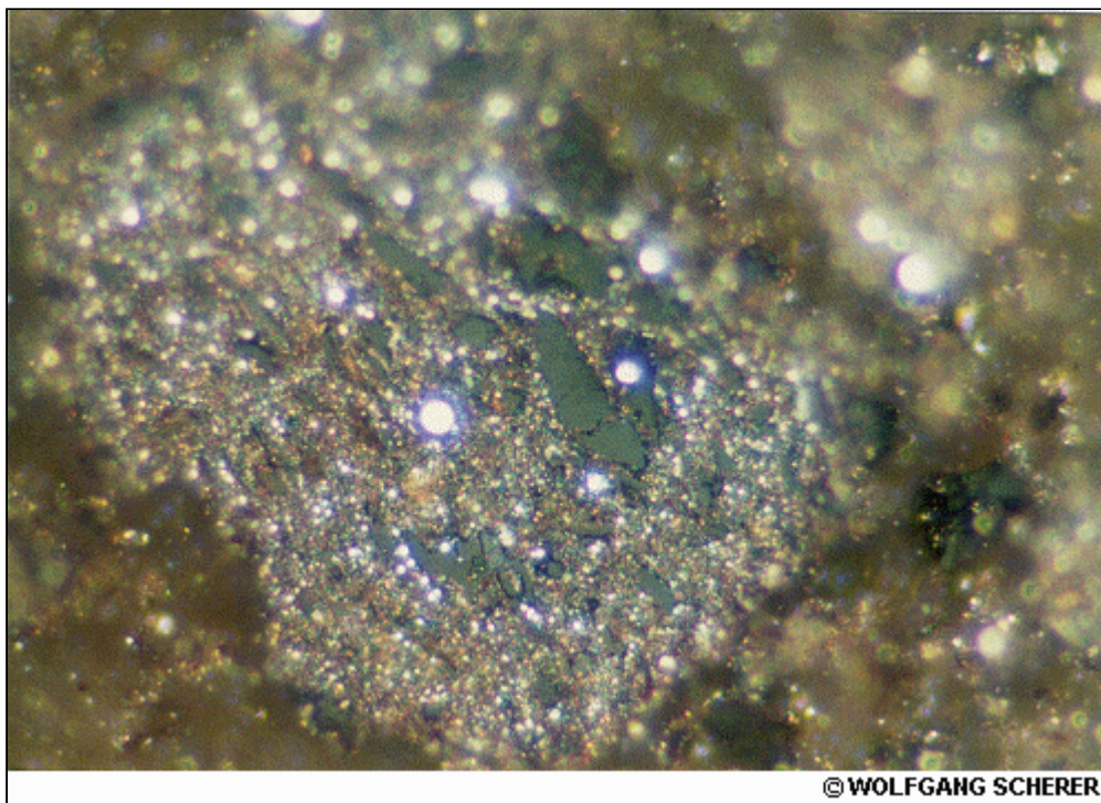
Sample ATP-30 Vitinitre and Framboidal pyrite
