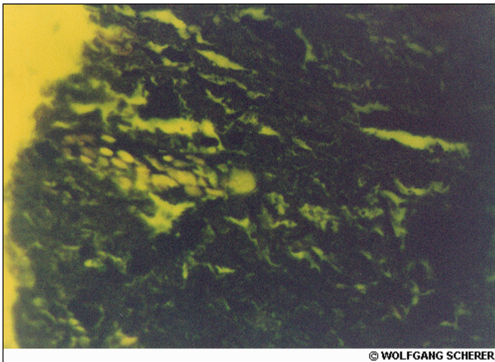
Sample ATP-30 Exinite and Exudinite-Fluorescent light
